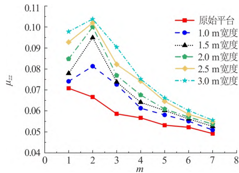
图7 带水平薄板模型不同衰减周期内 \mu_{zz} 变化 Fig.7 Damping coefficient \mu_{zz} changes of models with horizontal thin plates at different decay periods
