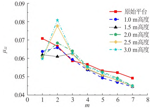
图9 带垂直薄板模型不同衰减周期内 \mu_{zz} 变化 Fig.9 Damping coefficient \mu_{zz} changes of models with vertical thin plates at different decay periods
